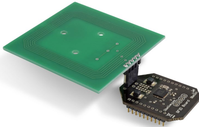
Figure : RFID/NFC module for 13.56 MHz and antenna
