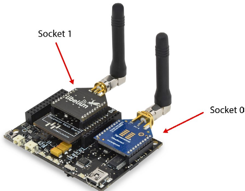
Figure : Wasp mote with XBee radio on socket 0 and Bluetooth module on socket 1
